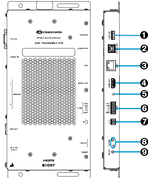
Side View, Right (DM-TX-4K-302-C Shown)
