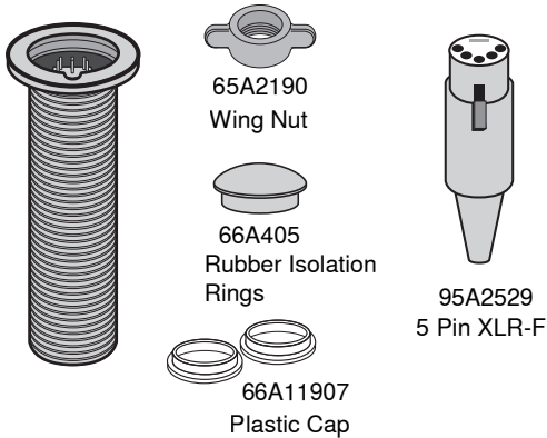
MX400SMP Surface Mount Kit
