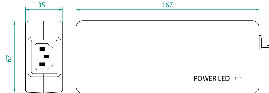
Power supply
